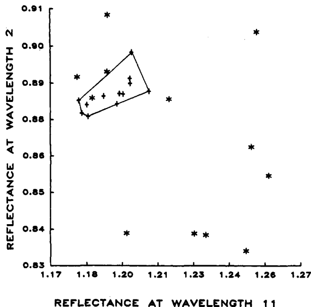
Figure 8. One of six orthogonal views of a four-dimensional space formed by taking Datriil-capsule spectra at four wavelengths for training-set capsules (+) and NaCN-containing capsules (*). This figure shows the smallest convex polygon that can completely surround the training-set spectral points.
