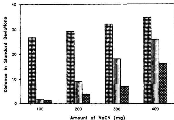
Figure 6. Datriil capsules read with the colored end up in the reflector cone, containing approximately 100, 200, 300, and 400 mg of NaCN packed in three configurations: in the colored end (crosshatch), in the white end (vertical line), and mixed throughout the capsule (diagonal crosshatch). The distance in standard deviations is given in terms of the training set of unadulterated Datriil capsules in the direction of the NaCN-containing capsule.
