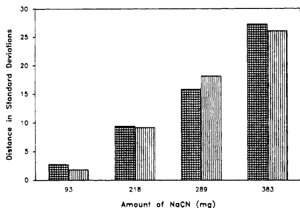
Figure 4. The theoretical and actual response for a contaminant packed in the lower end of a Datriil capsule in the conical reflector. The first bar (crosshatch) represents the scaled NaCN theoretical distance (from eq 3) response of the BEAST for an adulterated capsule filled from the bottom to the top in 100-mg steps. The second bar (vertical lines) represents the actual response of the BEAST for NaCN packed into the white (bottom) end of a Datriil capsule.
