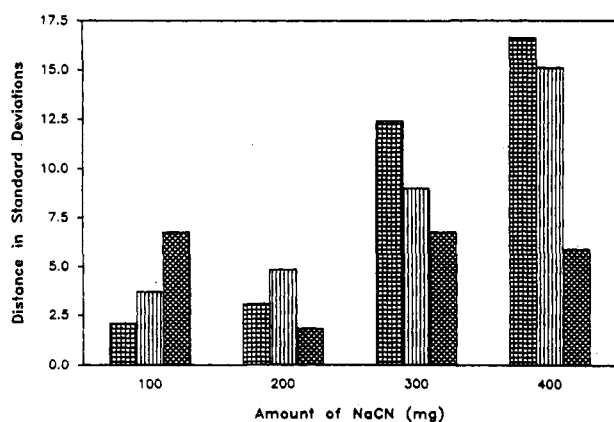
Figure 7. Datriil capsules read with the colored end down in the reflector cone (white end up), containing approximately 100, 200, 300, and 400 mg NaCN packed in three configurations: in the colored end (crosshatch) in the white end (vertical lines), and mixed throughout the capsule (diagonal crosshatch). The distance in standard deviations is given in terms of the training set of unadulterated Datriil capsules in the direction of the NaCN-containing capsule. The seemingly anomalous 100 mg "mixed" reading is probably the result of particle-size noise from, for instance, a large NaCN crystal against the blue end of the capsule wall.
